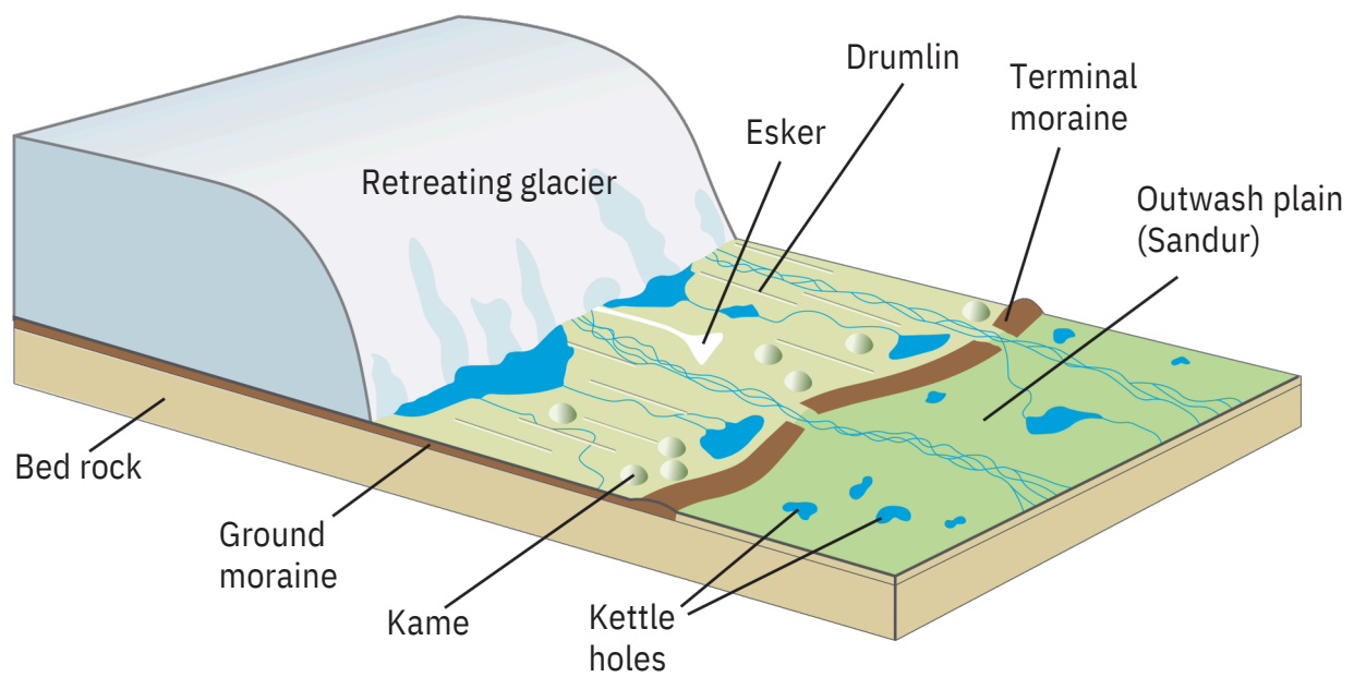
Figure 2b A glacial landscape
