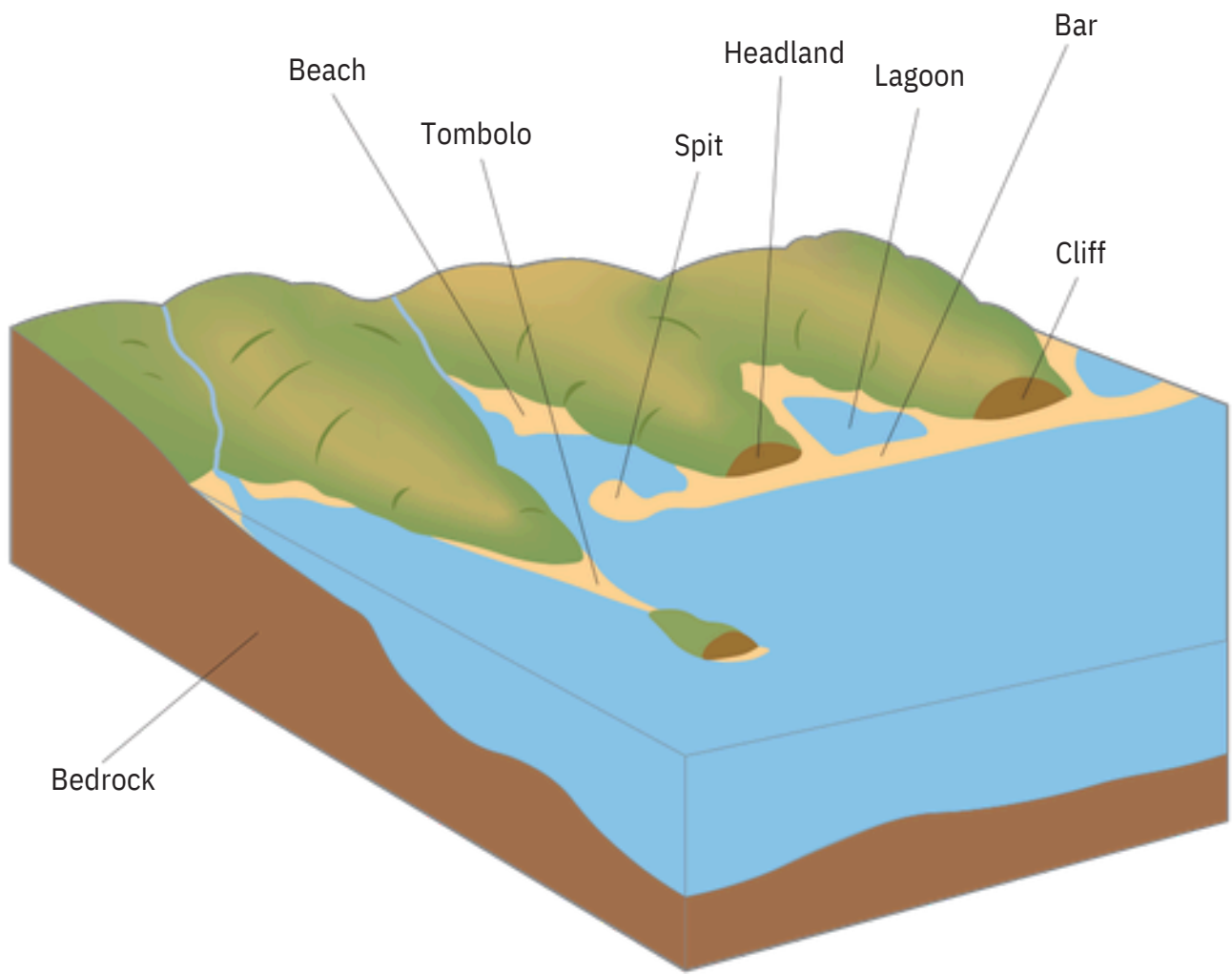
Figure 3b A coastal landscape
