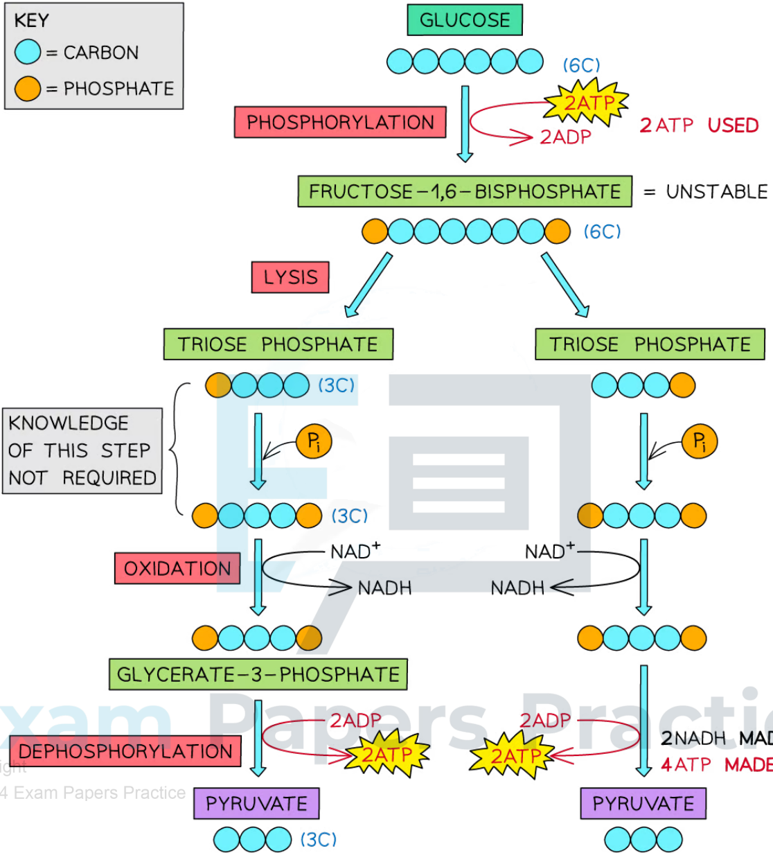
Glycolysis, the formation of two pyruvate molecules from one glucose sugar molecule
