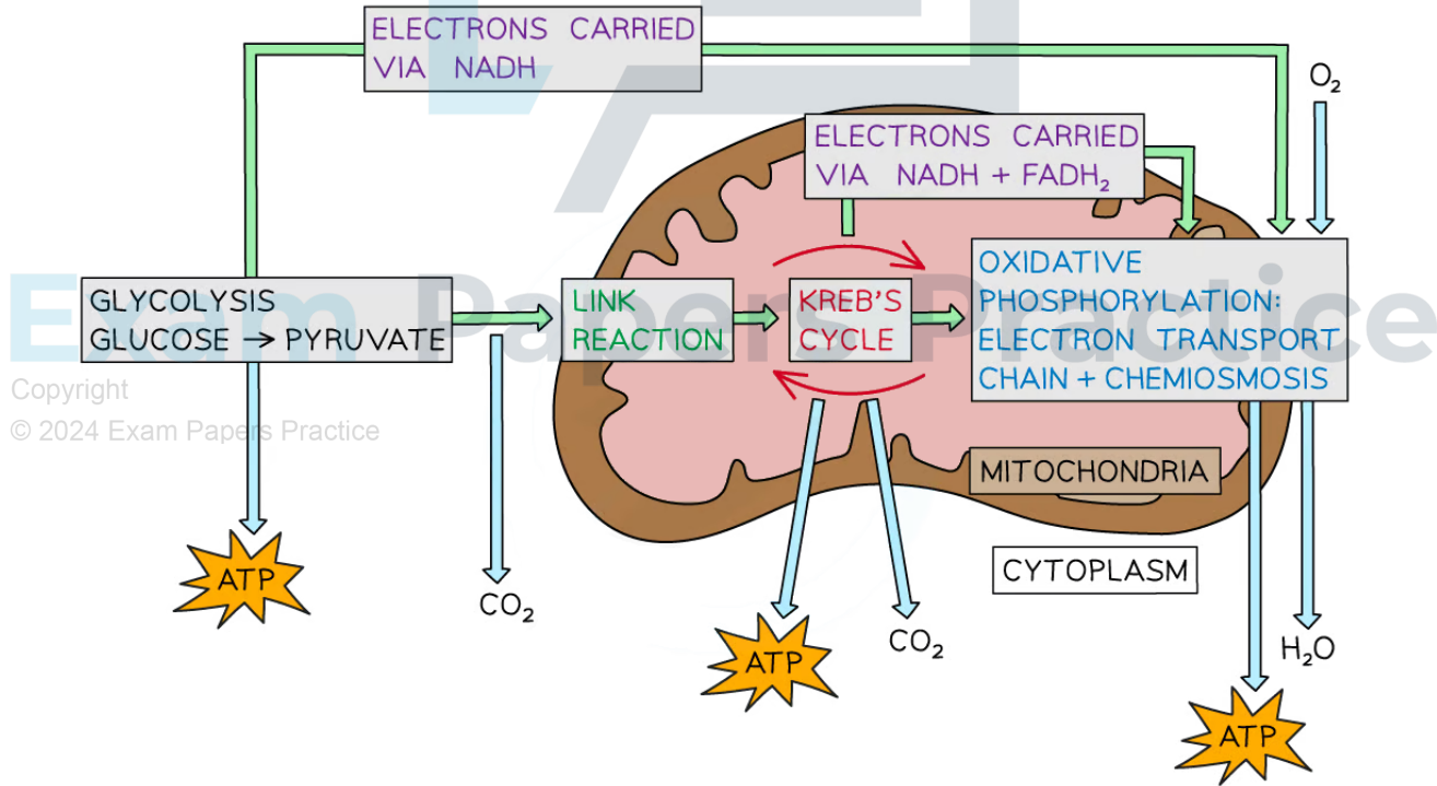
Overview of the four stages of aerobic respiration
