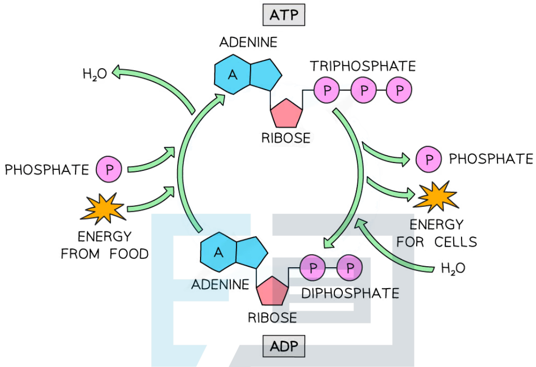
The cyclic formation of ATP from ADP by phosphorylation
