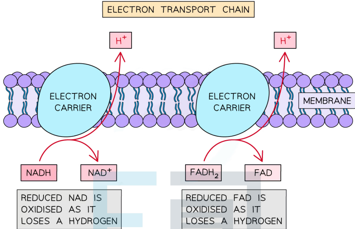
Identifying oxidation in the electron transport chain
