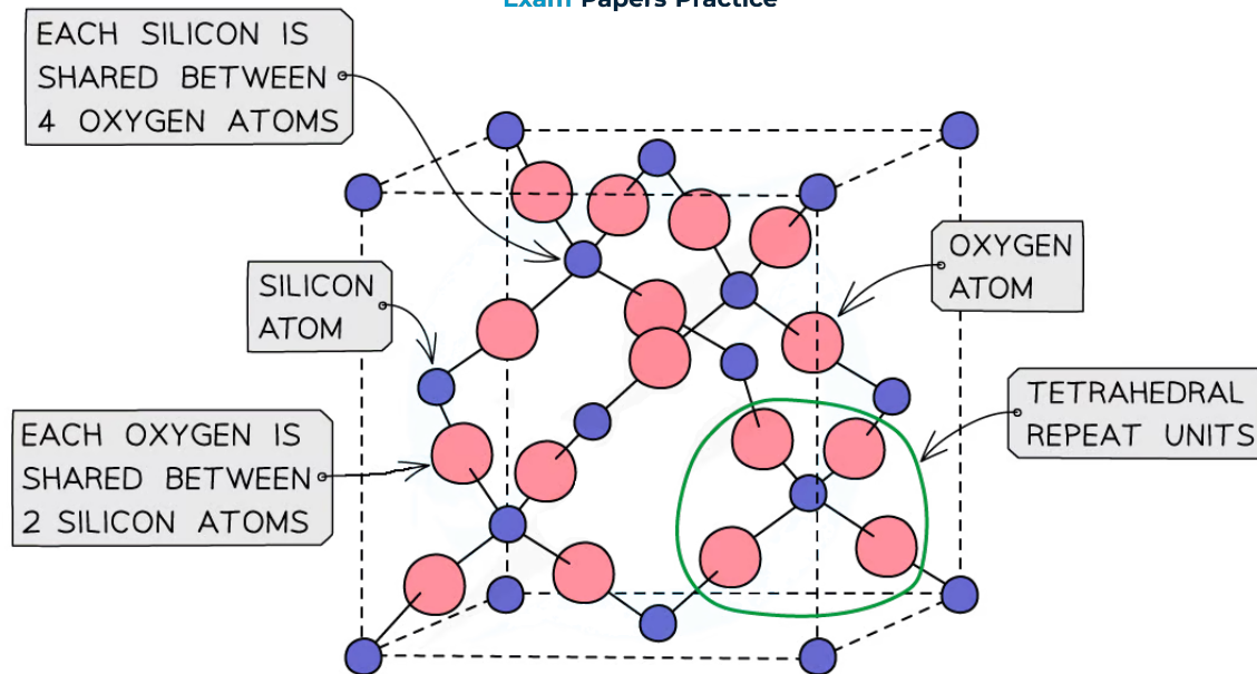
SILICON (IV) OXIDE ( \text{SiO}_2 )
