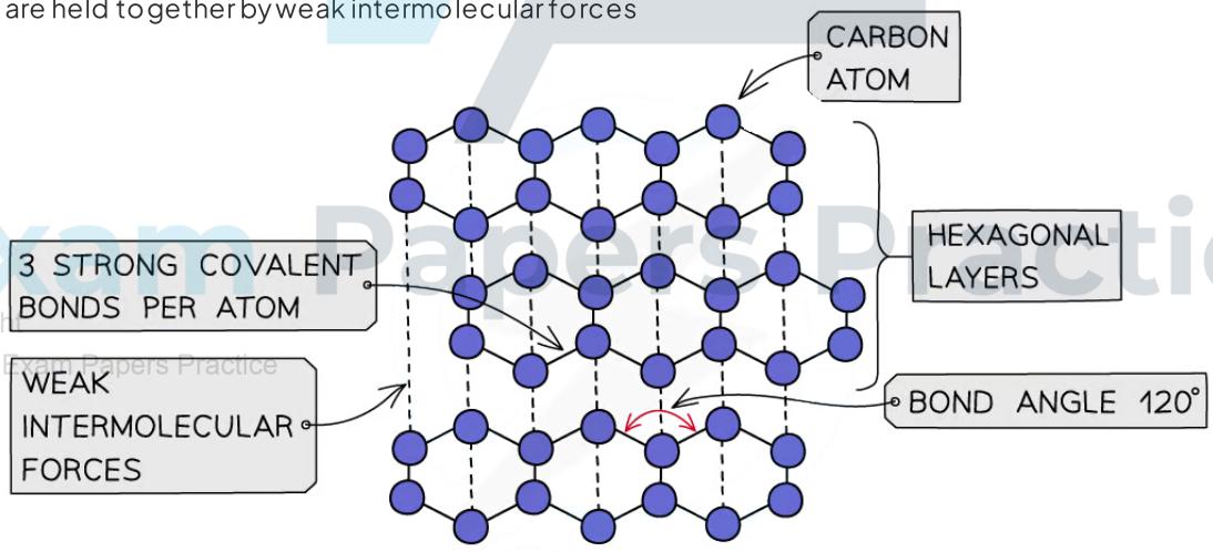
GRAPHITE (CARBON)
