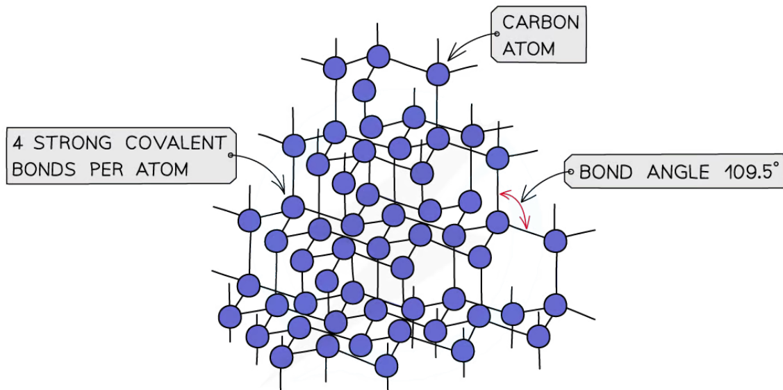
DIAMOND (CARBON)
