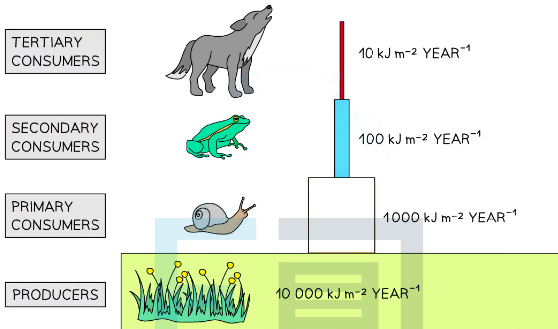
The energy stored in the biomass of organisms can be represented by a pyramid of energy
