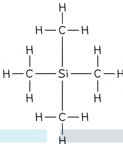
The displayed formula of tetramethylsilane
