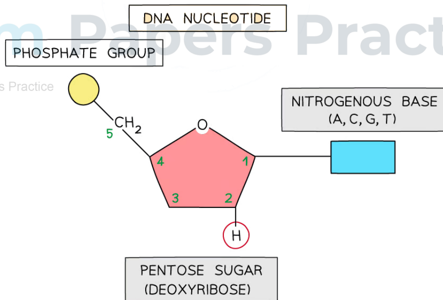
An RNA nucleotide compared with a DNA nucleotide
