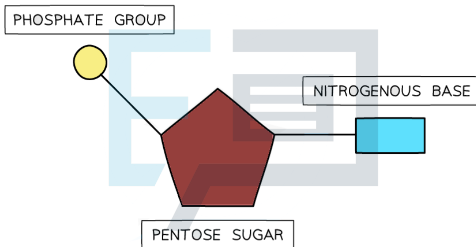
The basic structure of a nucleotide
