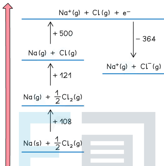
Drawing a Born-Haber cycle step 3 – creating the gaseous ions
